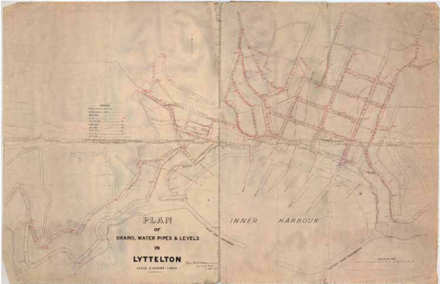
Plan of drains, water pipes and levels in Lyttelton, 1908.
